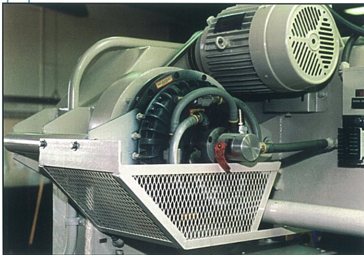
A new Wichita clutch installed on a Press Brake.
